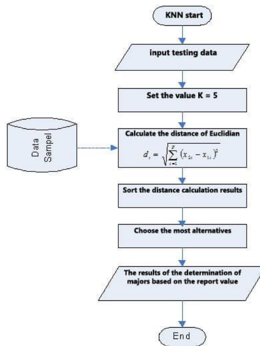
Fig 3: KNN Flowchart
